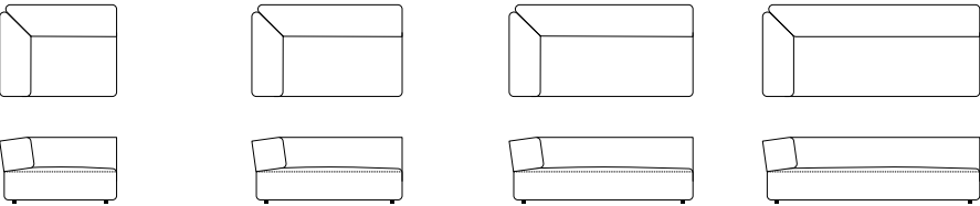
9THI301 L140 P110 H67 9THI302 L180 P110 H67 9THI303 L220 P110 H67 9THI304 L260 P110 H67
