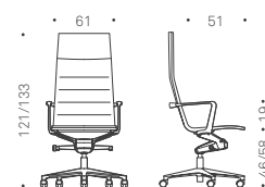
tilting support
